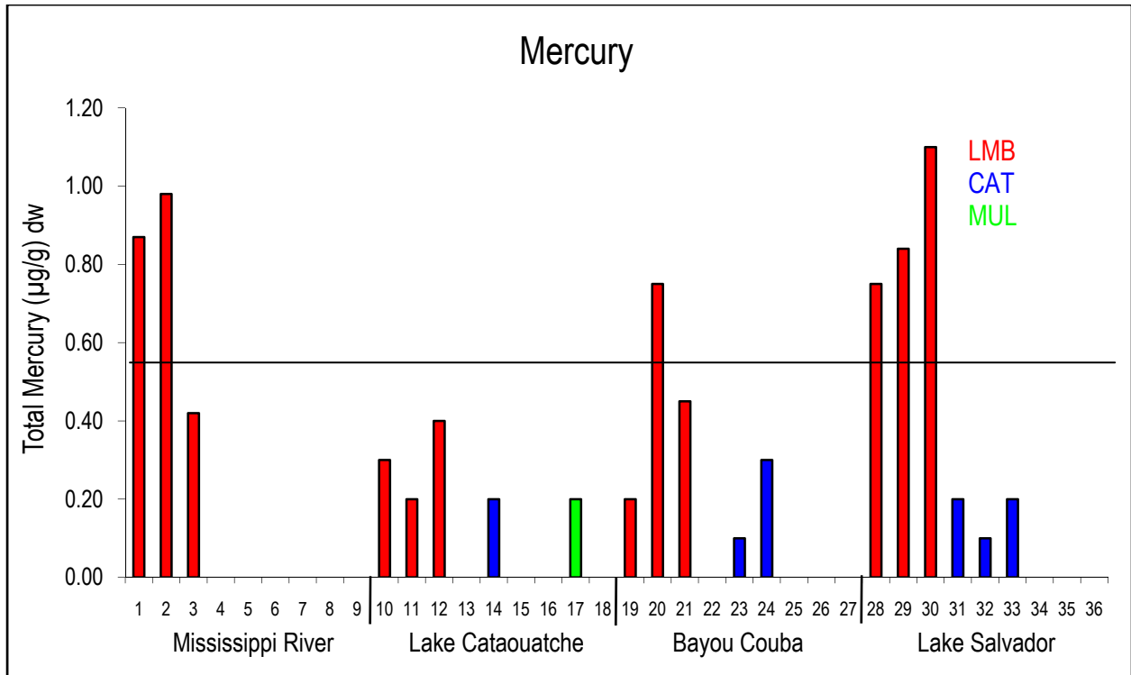
Figure 20A. Mercury in dry weight from largemouth bass (LMB; Micropterus salmoides ), blue catfish (CAT; Ictalurus furcatus ), and striped mullet (MUL; Mugil cephalus ) collected from Davis Pond postdiversion sites from December 2007 through February 2009. The lower detection limit was 0.1 parts per million. The horizontal line represents the 85th percentile in dry weight from the National Contaminant Biomonitoring Program (Schmitt and Brumbaugh, 1990); for mercury it is 0.59 micrograms per gram ( \mu\text{g/g} ).
